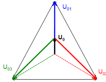
Fig.2 Vectors of phase voltage and the zero voltage vector
