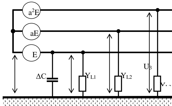
Fig.1 Simple circuit for the calculation
